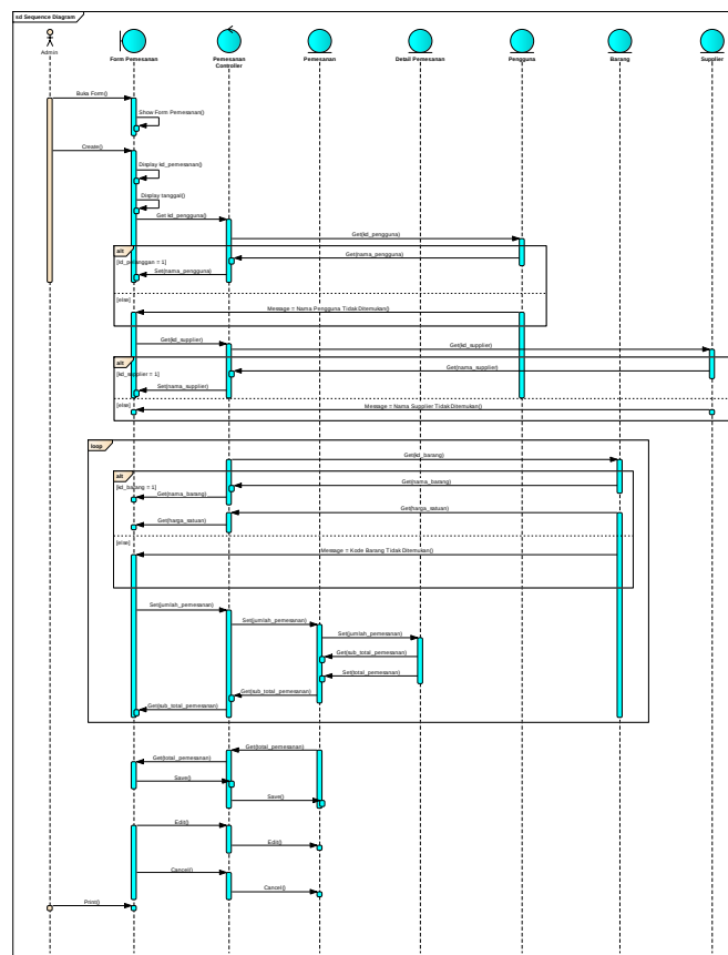
Gambar 5. Sequence Diagram.
