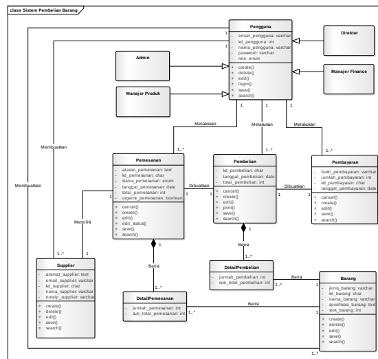
Gambar 4. Class Diagram.
